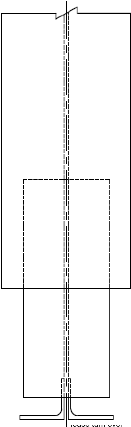
BEAM-TO-BEAM CONNECTIONSCALE 1:5
