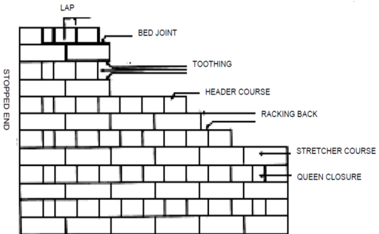
FRONT ELEVATION OF ENGLISH BOND SCALE 1:10
