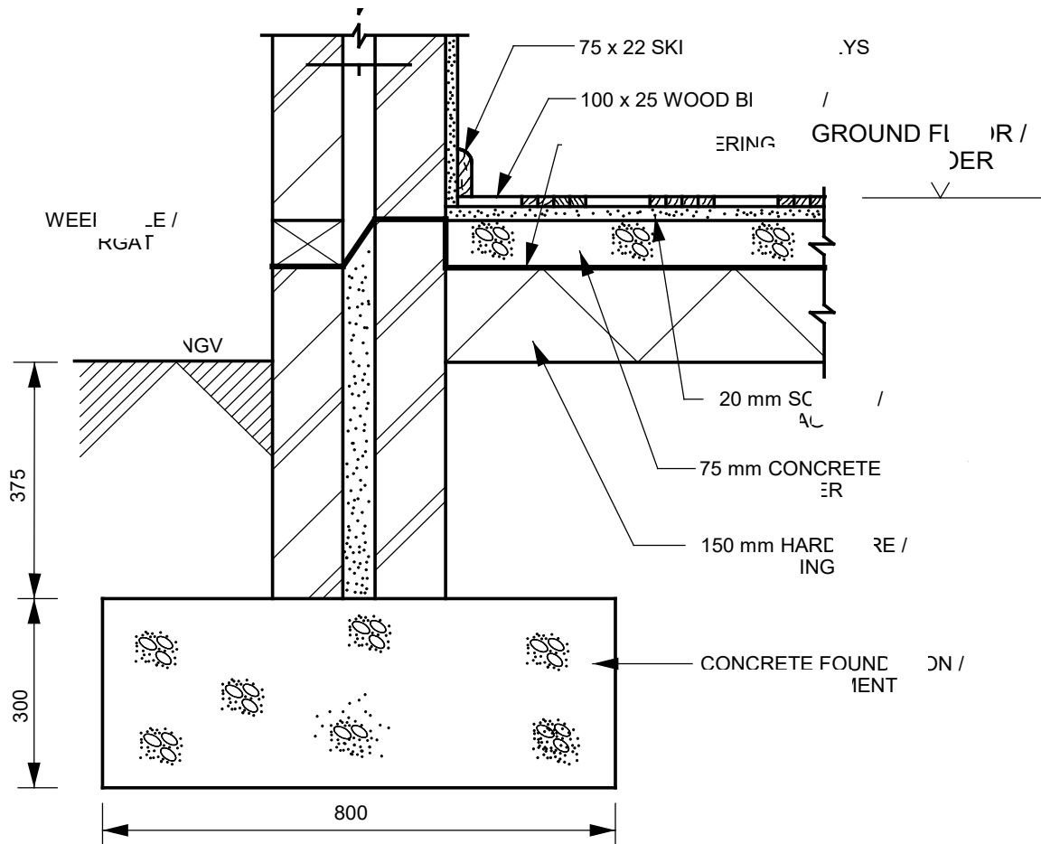
VERTICAL SECTION THROUGH THE GROUND AND FOUNDATION SCALE 1:10
