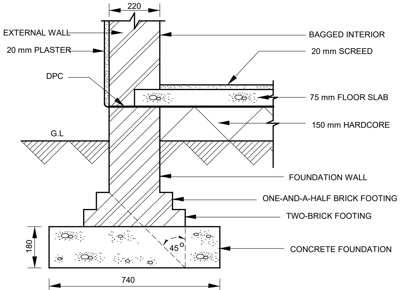
VERTICAL SECTION THROUGH EXTERNAL WALL AND FOUNDATION SCALE 1:10
