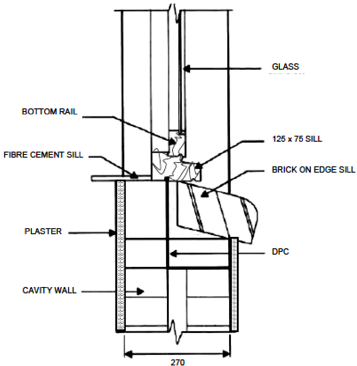
VERTICAL SECTION THROUGH BOTTOM CASEMENT WINDOW FRAME SCALE 1:5
