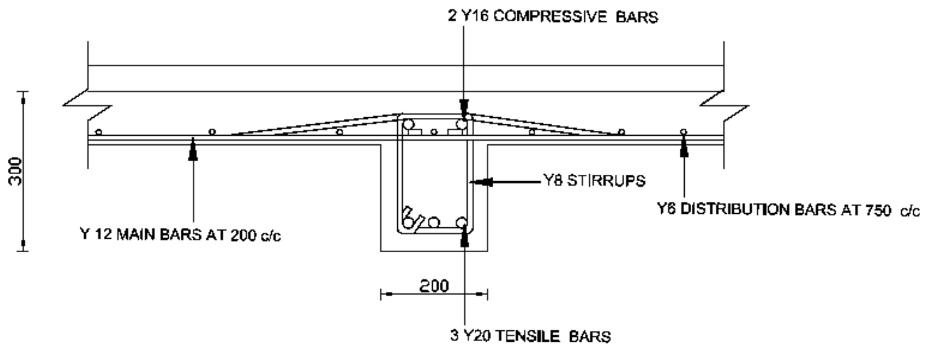
VERTICAL CROSS SECTION THROUGH T-BEAM SCALE 1:10
