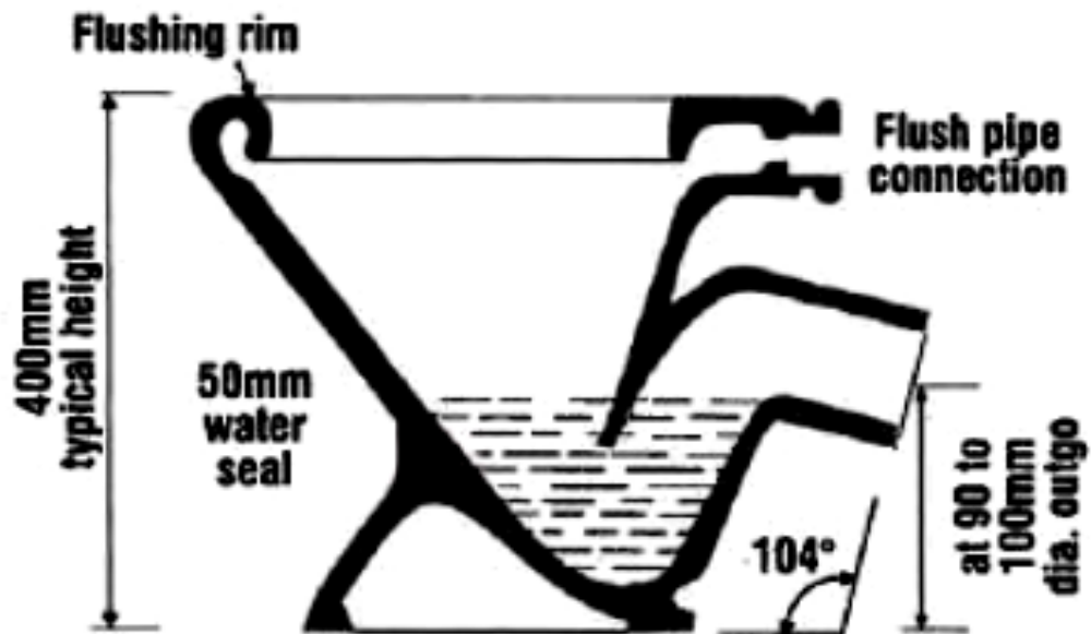
VERTICAL SECTION THROUGH FLUSHING SYSTEM
