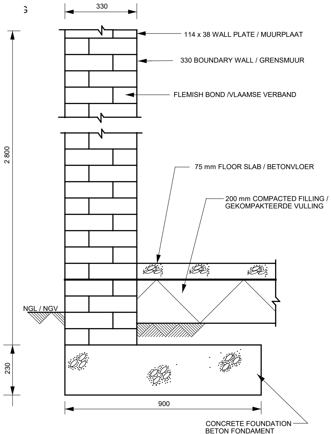
VERTICAL SECTION THROUGH BOUNDARY BUILT IN FLEMISH BOND SCALE 1 : 10
