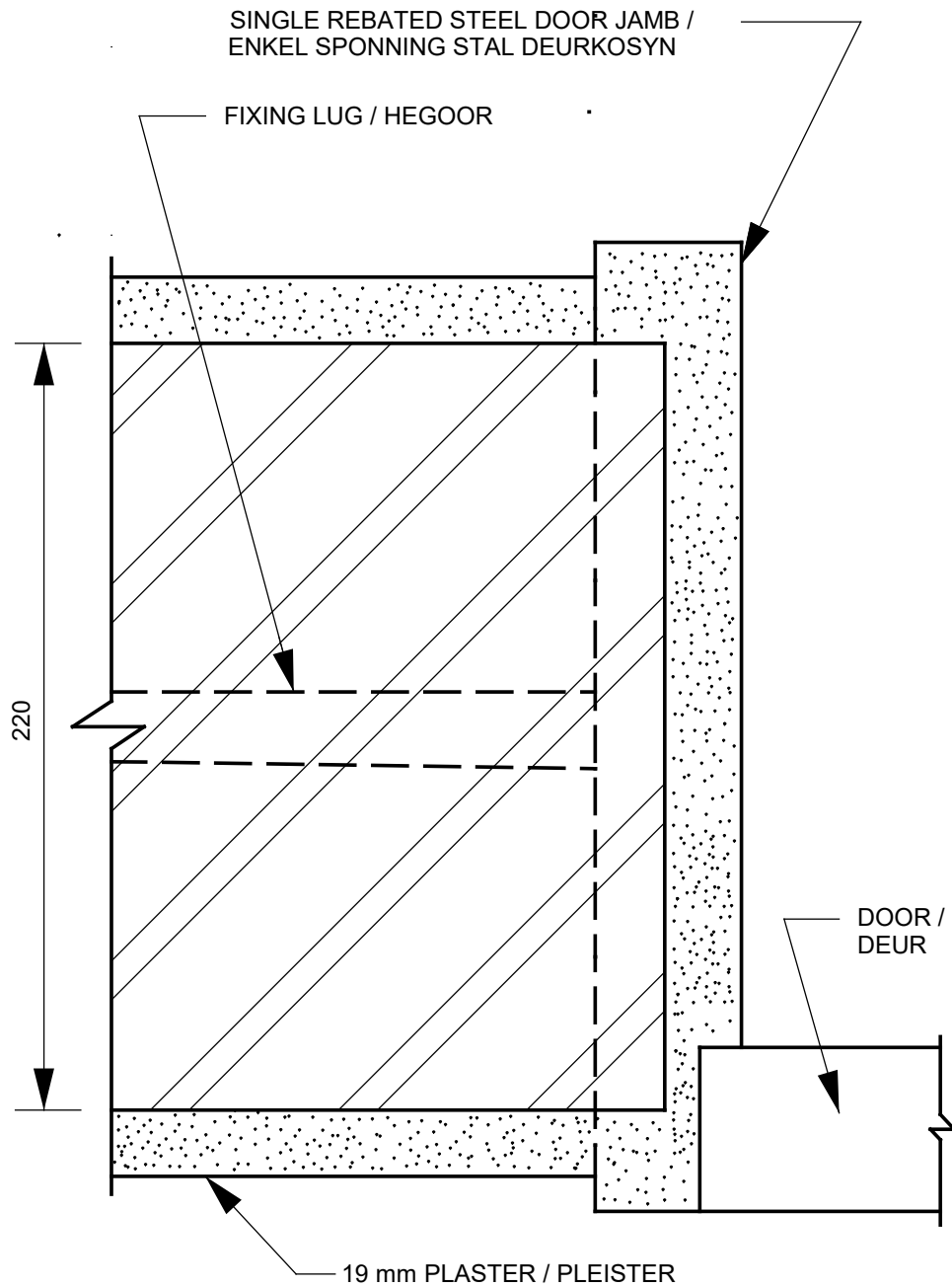
HORIZONTAL SECTION THROUGH A STEEL DOOR JAMB SCALE 1 : 2
