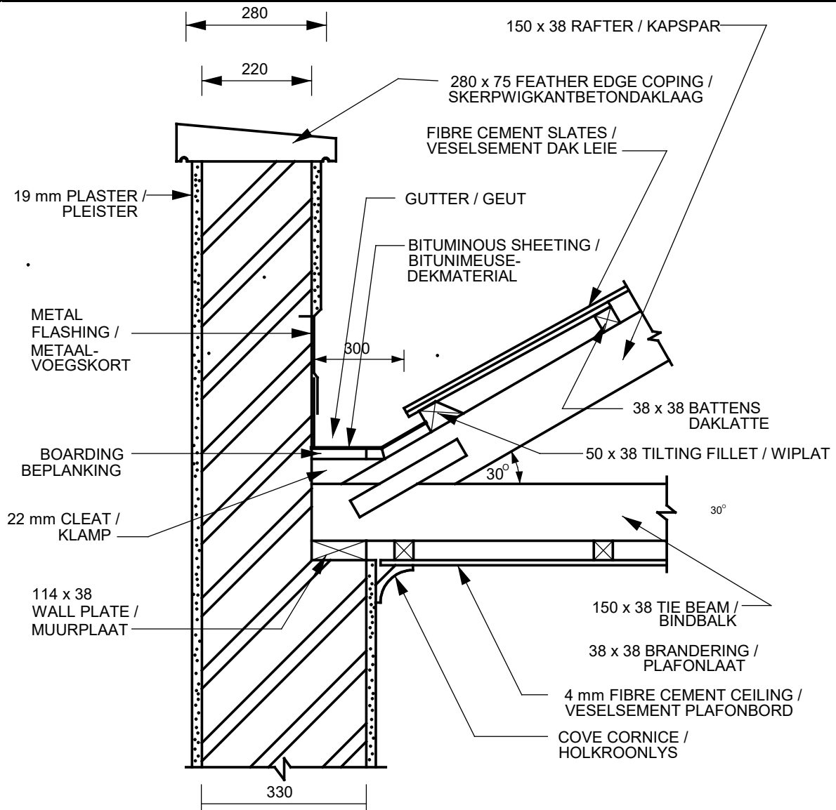
VERTICAL SECTION THROUGH A PARAPET GUTTER SCALE 1 : 10
