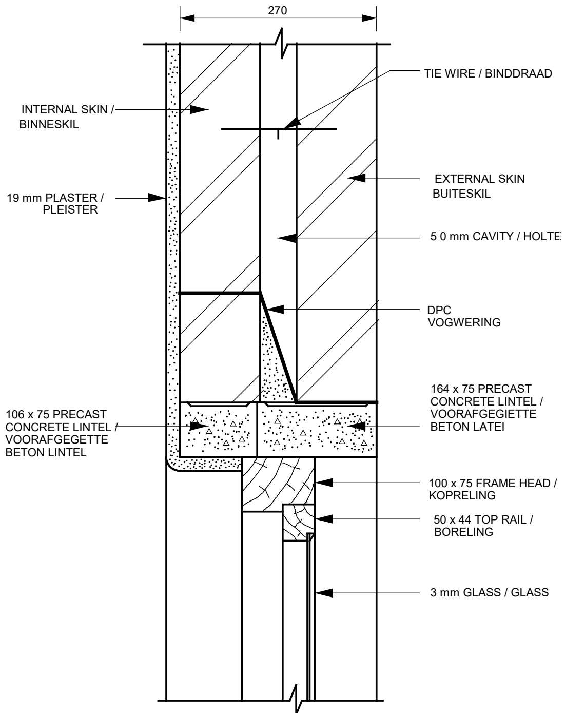
VERTICAL SECTION THROUGH THE TOP OF FRAME AND PRECAST CONCRETE LINTEL SCALE 1 : 5
