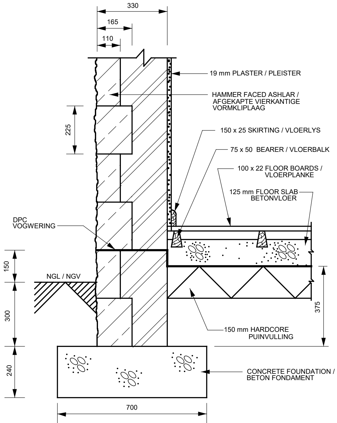
VERTICAL SECTION THROUGH A STONE-FACED WALL SCALE 1 : 10
