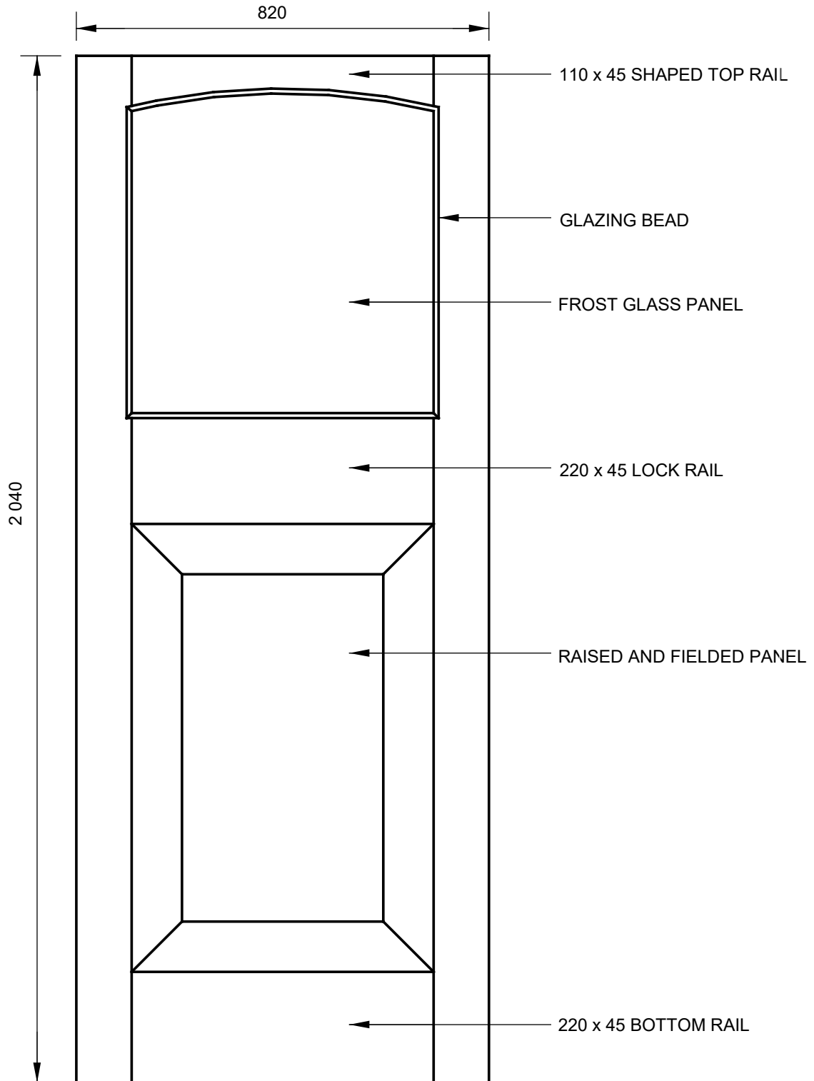
OUTSIDE VIEW OF DOOR SCALE 1:10
