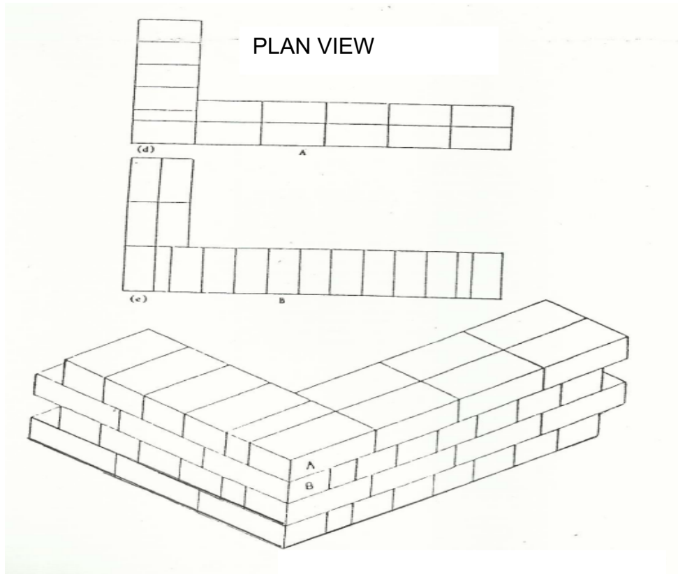
ISOMETRIC VIEW
