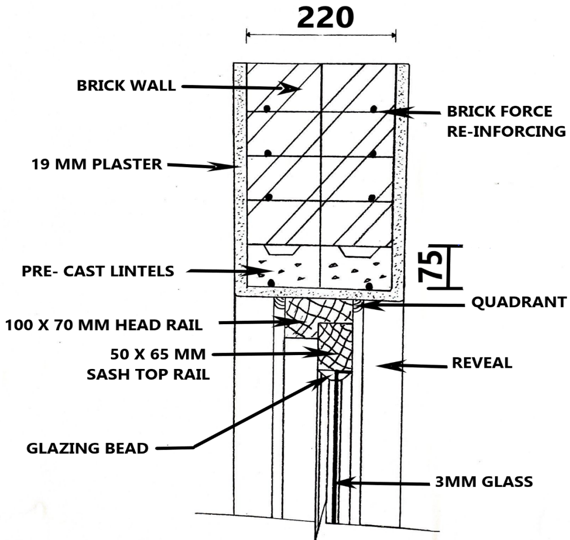
VERTICAL SECTION THROUGH LINTEL AND TIMBER RAIL SCALE 1:10
